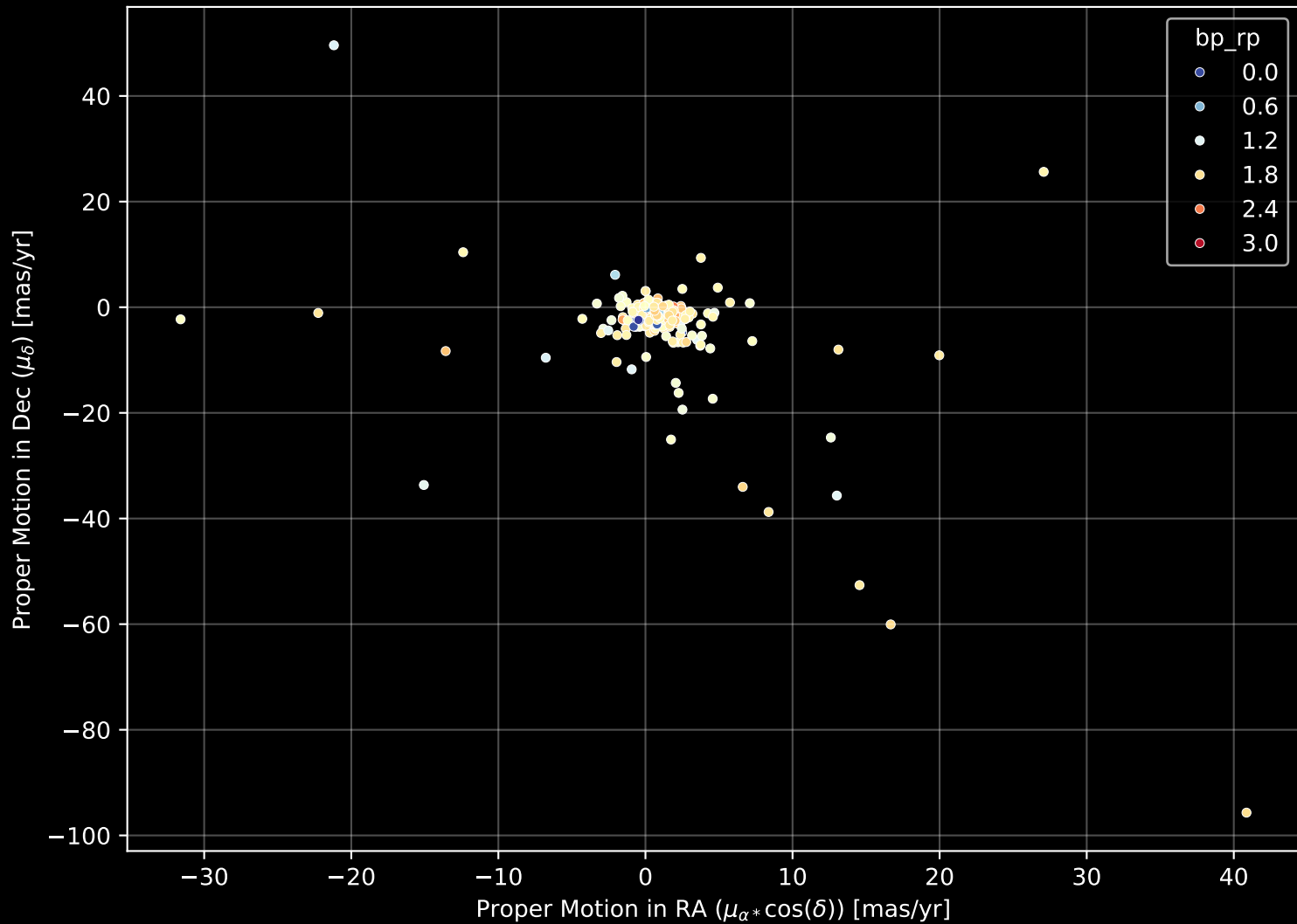
APOGEE DR17 Field: [165+00] Proper Motion Diagram (n= 430)
