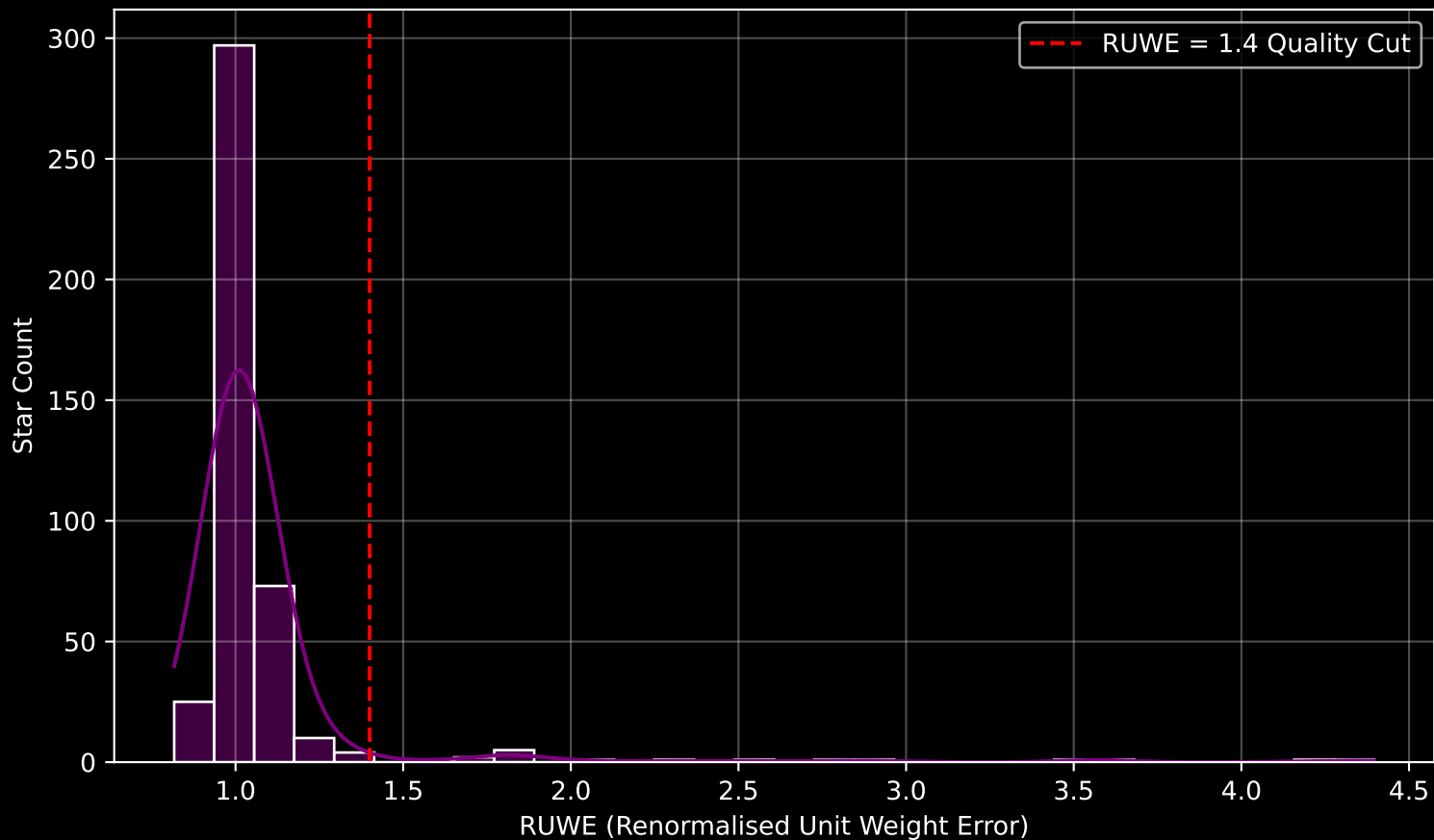
GAPOGEE DR17 Field [165+00] RUWE Distribution (n= 426)
