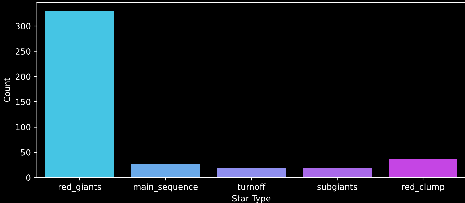
APOGEE DR17 Field: [165+00] Count plot of Star Type
