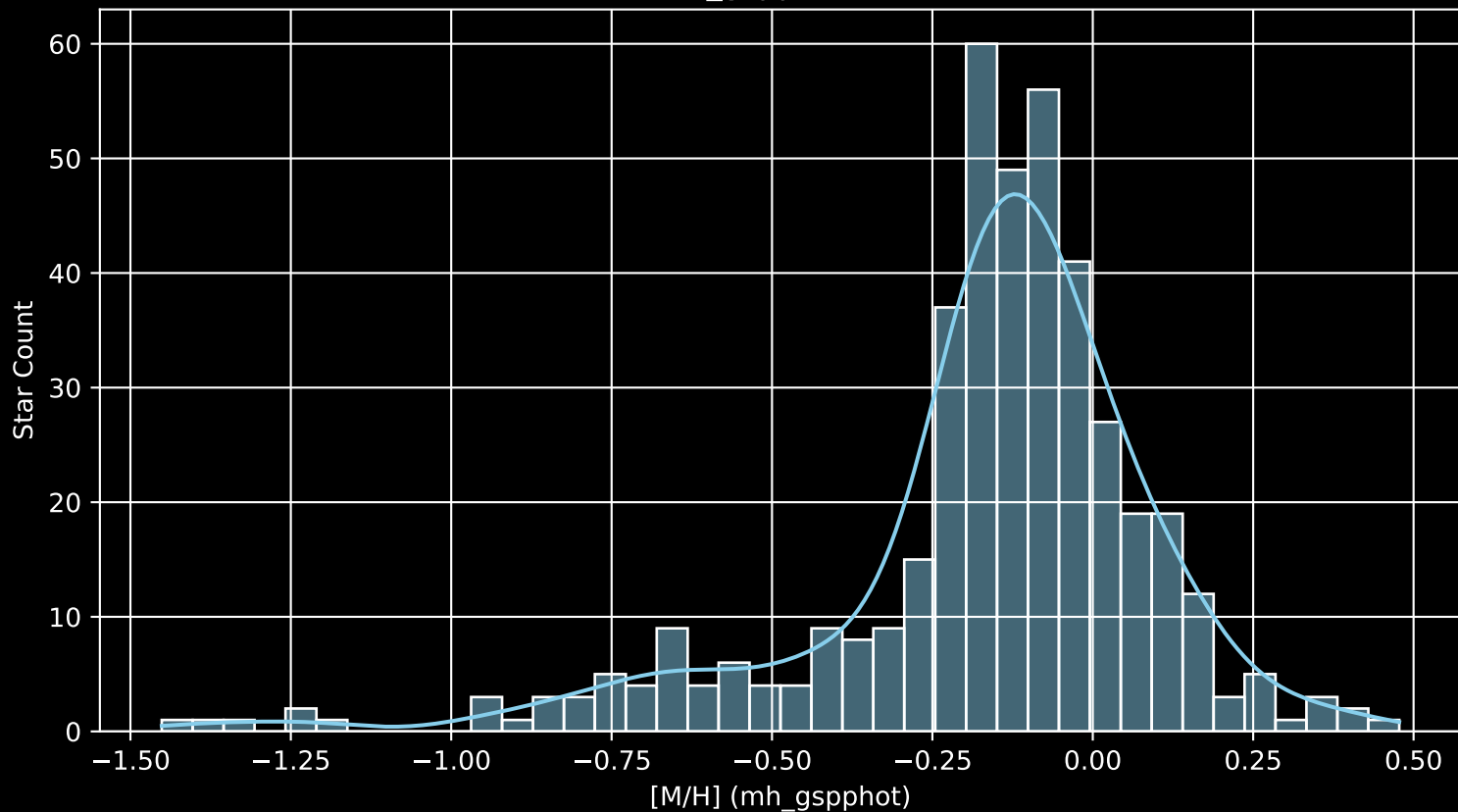
APOGEE DR17 Field: [165+00 [M/H] (mh_gspphot) (n= 428)
