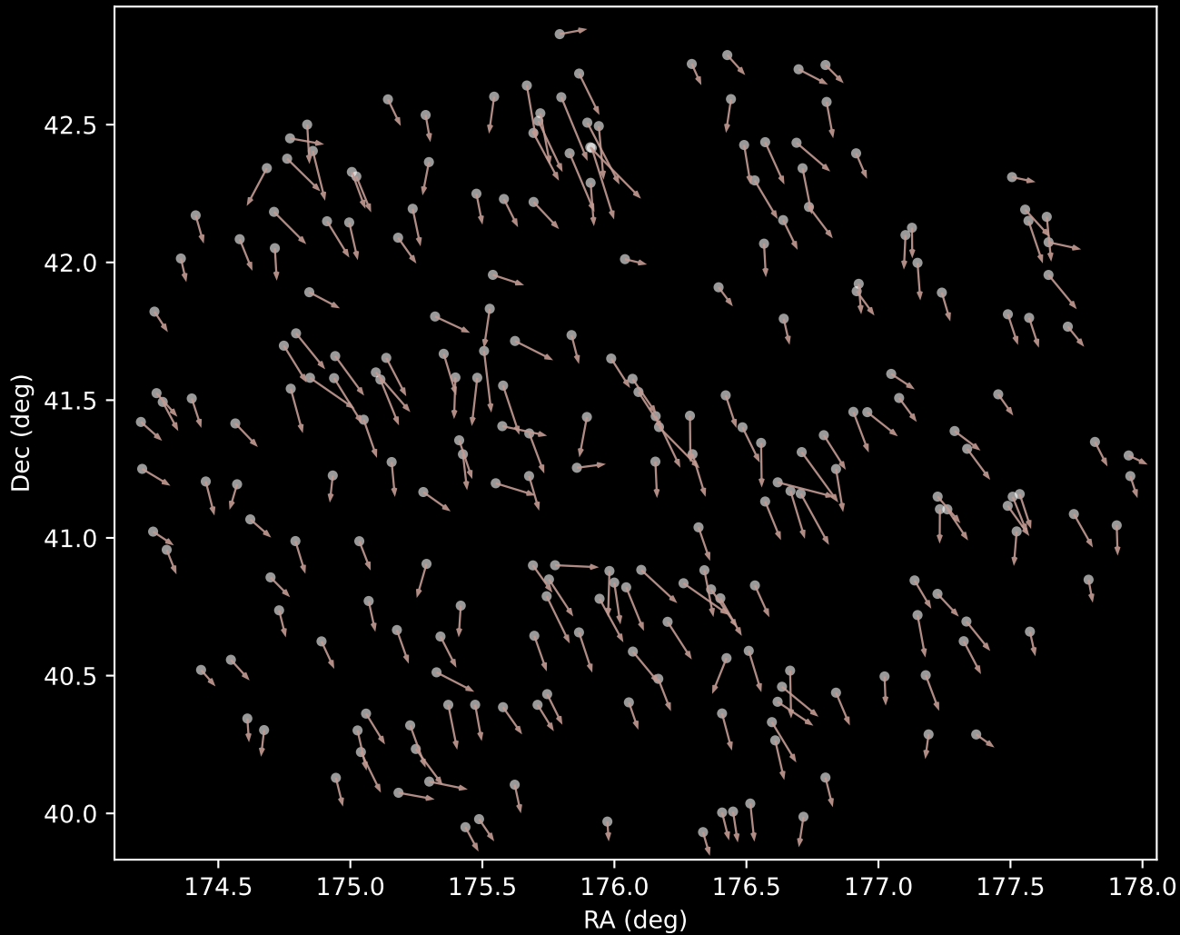
APOGEE DR17 Cluster 11 Proper Motion Vectors (n=229)
