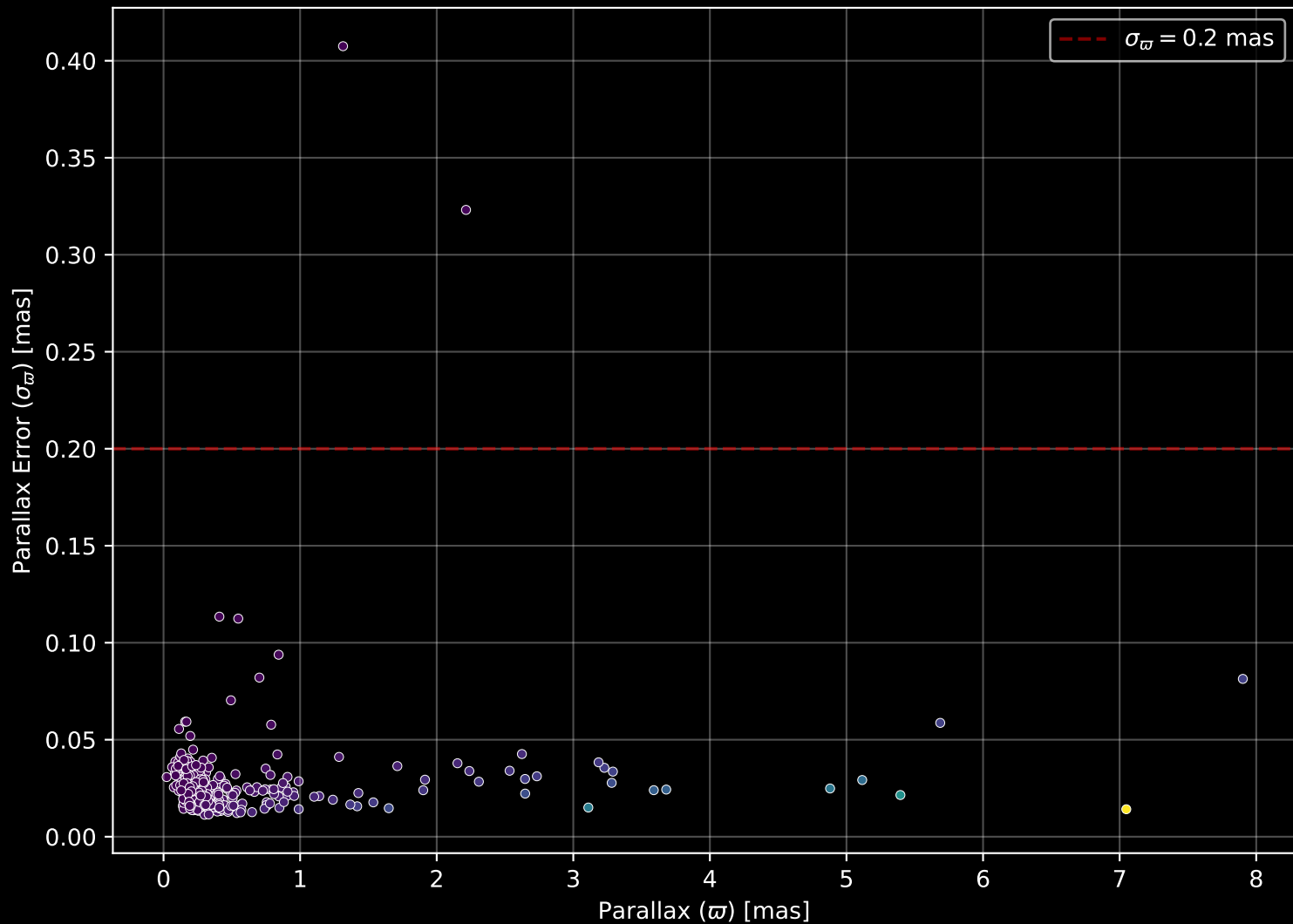
APOGEE DR17 Field: [165+00] Parallax Quality (n= 430)
