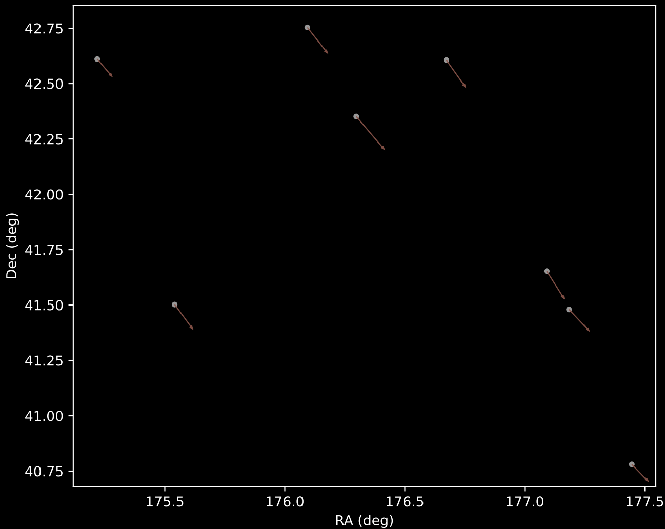
APOGEE DR17 Cluster 10 Proper Motion Vectors (n=8)
